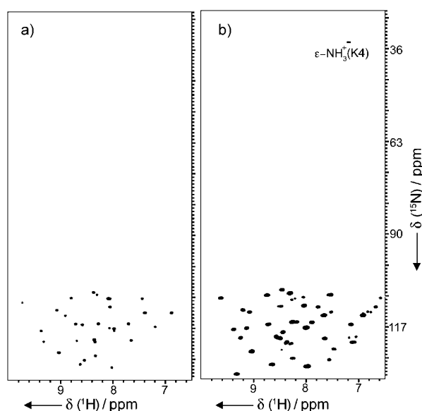
Figure 3. \epsilon -NH 3 + of Lys4 is protected from fast exchange with the solvent in trypsin-bound MCoTI-I. \{^1\text{H}, ^{15}\text{N}\} -HSQC spectra of free (a) and trypsin-bound MCoTI-I (b) were collected at room temperature with the ^{15}\text{N} -carrier position at 82 ppm and ^{15}\text{N} radio-frequency field strengths of 5.2 kHz for 90° and 180° pulses and 1.2 kHz for composite decoupling during acquisition.
